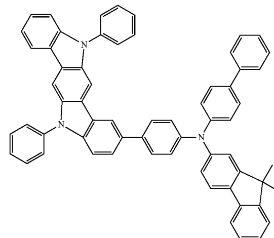
Compound 3
