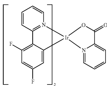
F 2 Irpq
