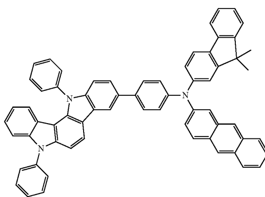
Compound 14
