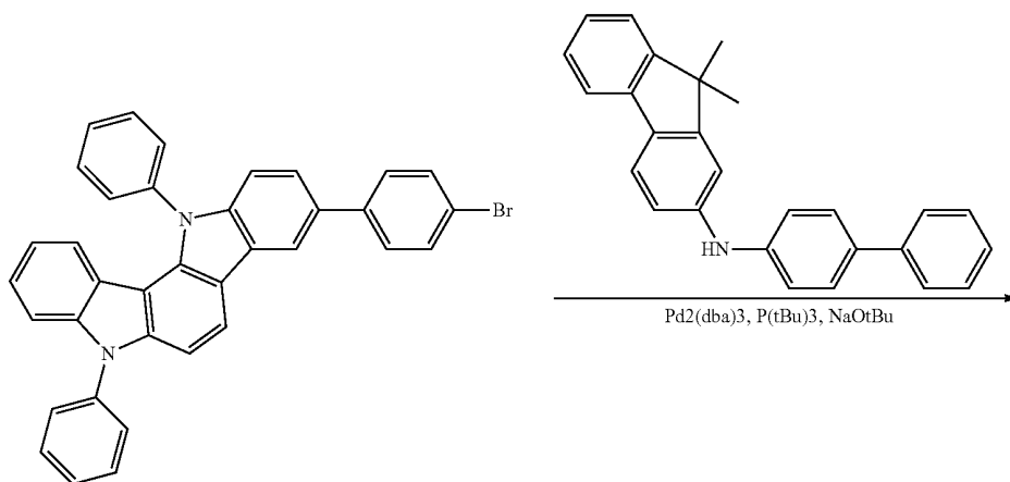
Reaction Scheme 4
