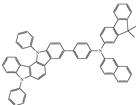
Compound 13
