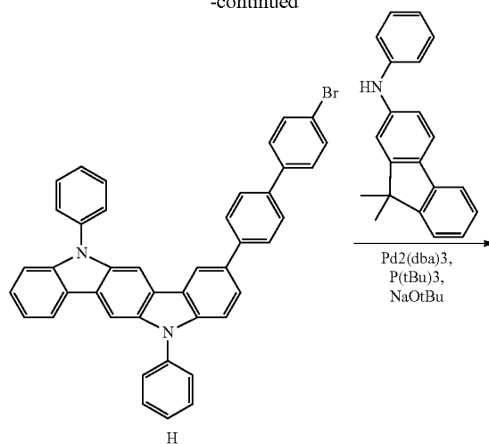
Compound 11
