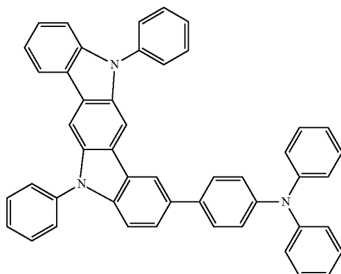
Compound 1
