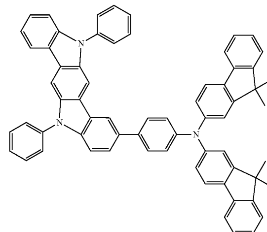
Compound 4
