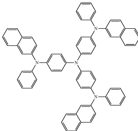
2T-NATA
