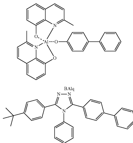
TAZ
