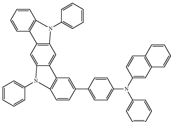
Compound 5
