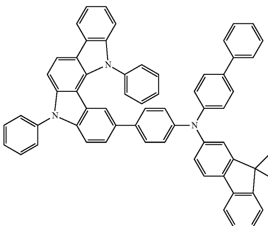
Compound 16
