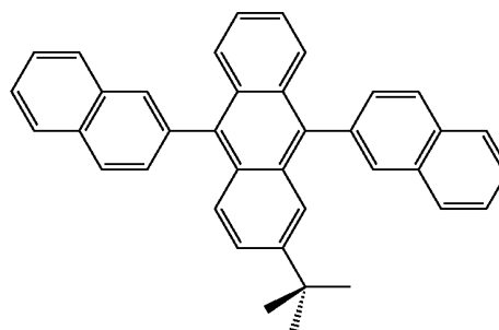
TBADN
