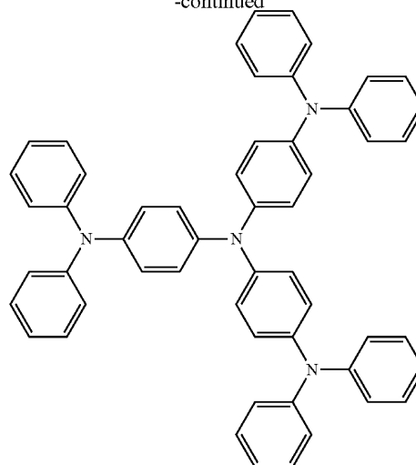
TDATA
