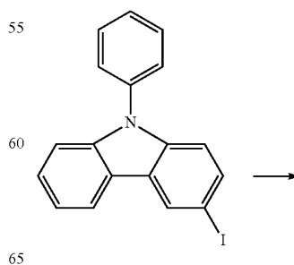
Reaction Scheme 8
