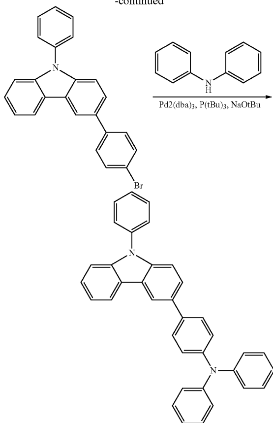
Compound B
