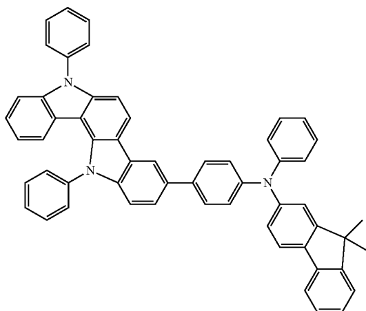
Compound 18
