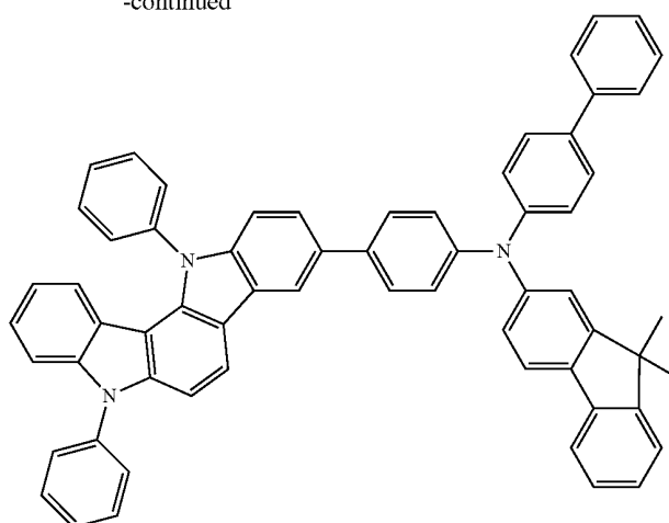
Compound 11
