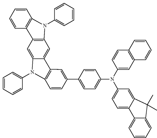
Compound 7
