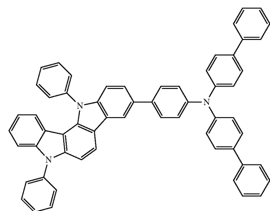
Compound 10
