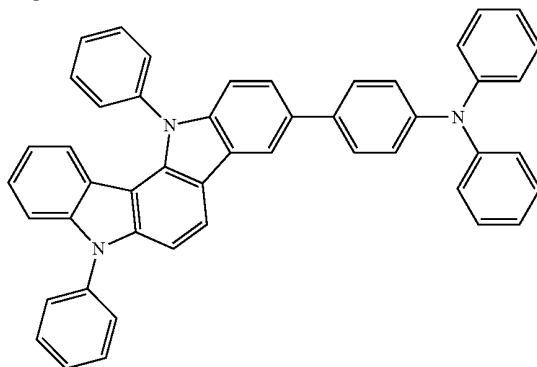
Compound 9
