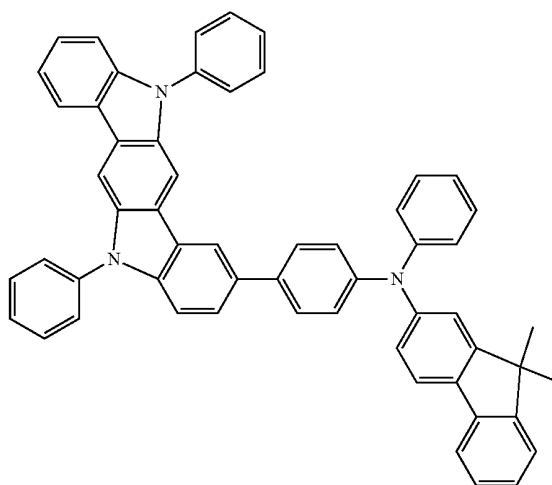
Compound 19
