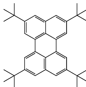
TBPc
