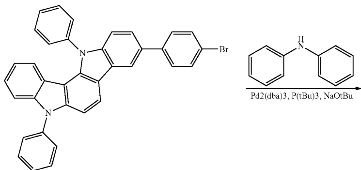
Reaction Scheme 3
