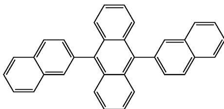
ADN
