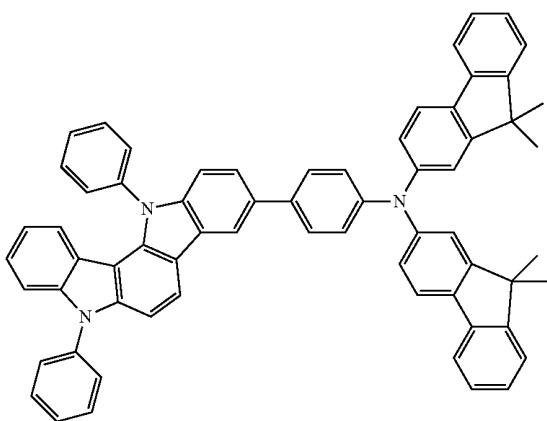
Compound 12
