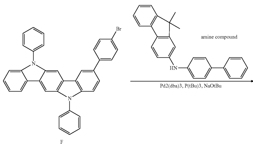
Reaction Scheme 2
