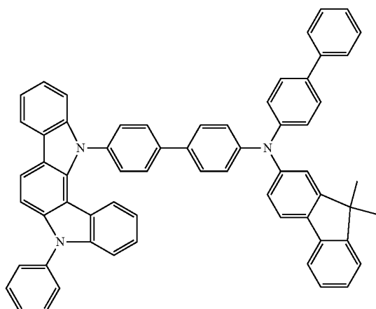
Compound 24
