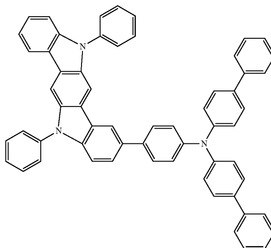
Compound 3
