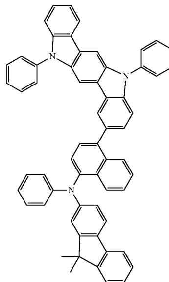
Compound 27
