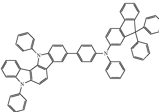
Compound 15
