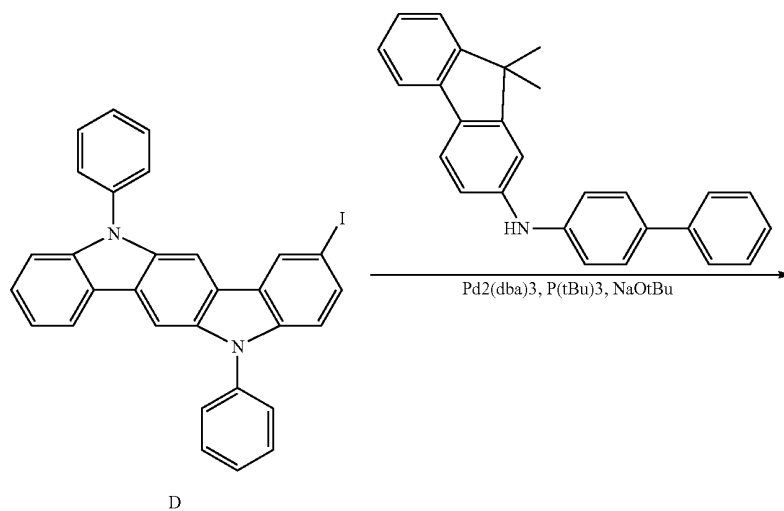
Reaction Scheme 7
