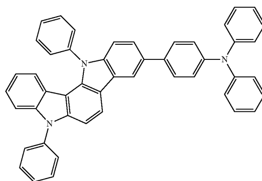
Compound 9
