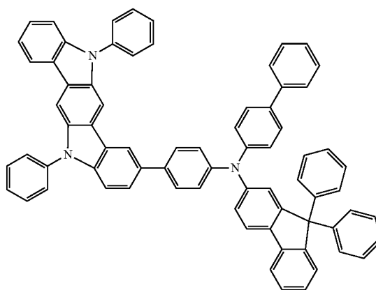
Compound 8
