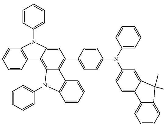
Compound 21
