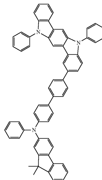
Compound 26
