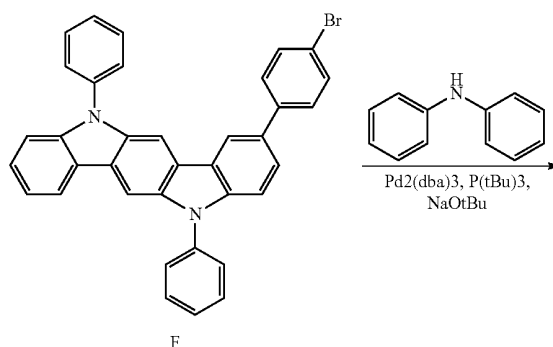
Reaction Scheme 1b
