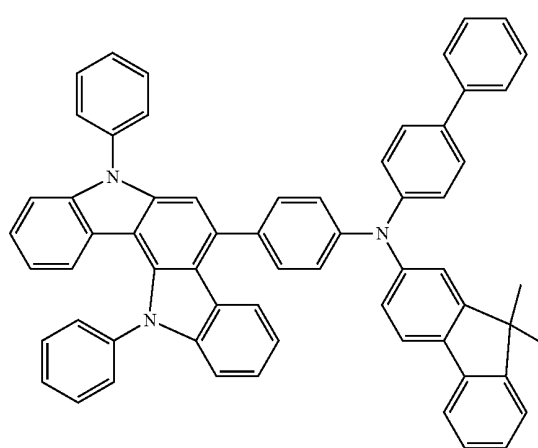
Compound 20
