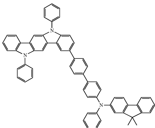
Compound 26
