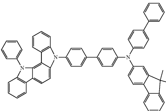
Compound 22
