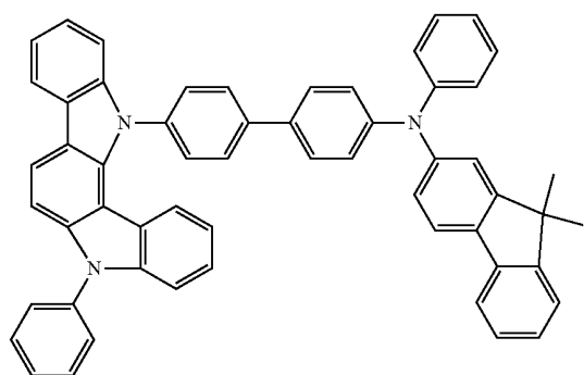
Compound 26
