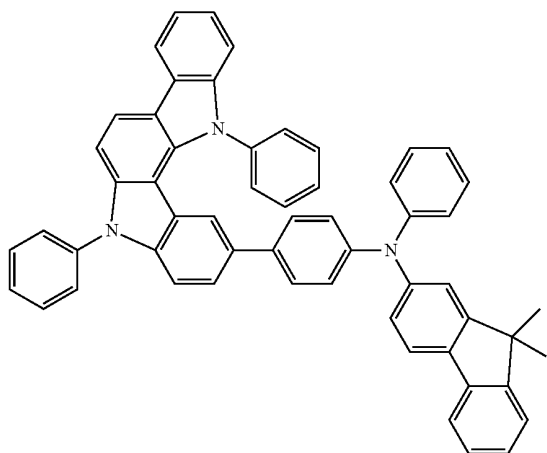
Compound 17
