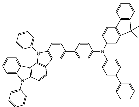
Compound 11
