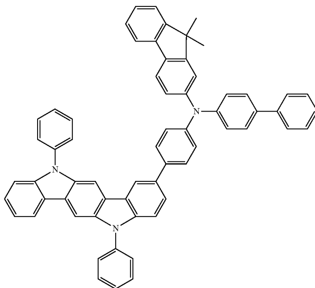
Compound 3
